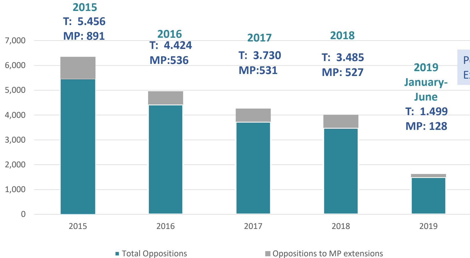
Total Oppositions vs. Total Oppositions to MP Extensions.
